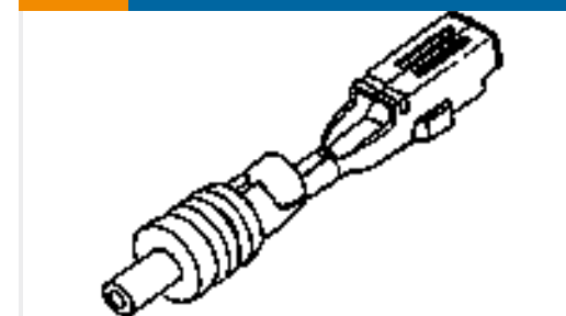
TE Part #1745032-1 2 POS. MCP2.8 CONNECTOR FOR IGNITION KEY
