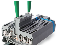
Test plug modules are directly plugged into the jumper contact slot of the current bar.
