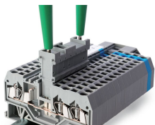
Test plug modules are directly plugged into the jumper contact slot of the current bar.
