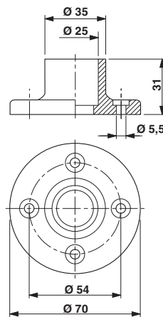
Dimensional drawing
