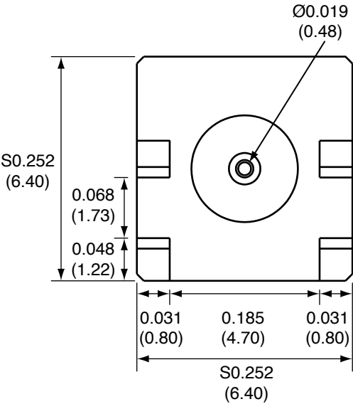
BACK VIEW
