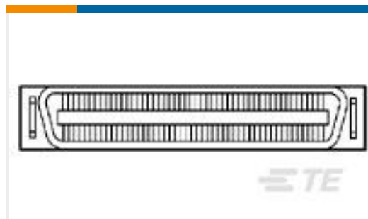
TE Part #5-5175473-6 .050CL,CHAMP,VERT PLUG,50 POSN
