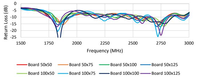
Return Loss for 2372112-1 (150mm) in Orthogonal Ground Plane Distance
