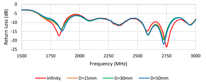
Return Loss for 2372112-1 (150mm) in Parallel Floating Metal Plate Distance (Left Side)
