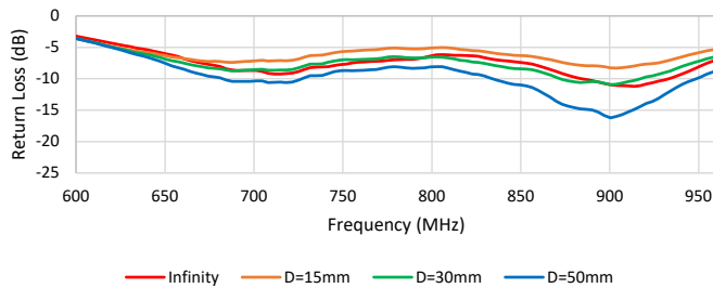
Return Loss for 2372112-1 (150mm) in Parallel Floating Metal Plate Distance (Centered)
