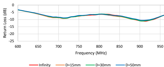
Return Loss for 2372112-1 (150mm) in Parallel Floating Metal Plate Distance (Right Side)
