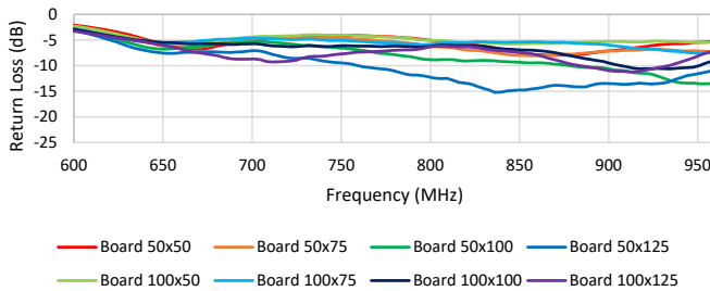
Return Loss for 2372112-1 (150mm) in Orthogonal Ground Plane Distance
