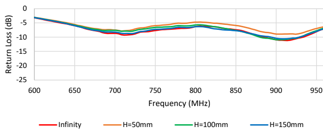
Return Loss for 2372112-1 (150mm) in Orthogonal Floating Metal Plate Distance (Centered)
