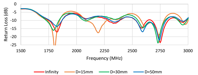
Return Loss for 2372112-1 (150mm) in Parallel Floating Metal Plate Distance (Centered)
