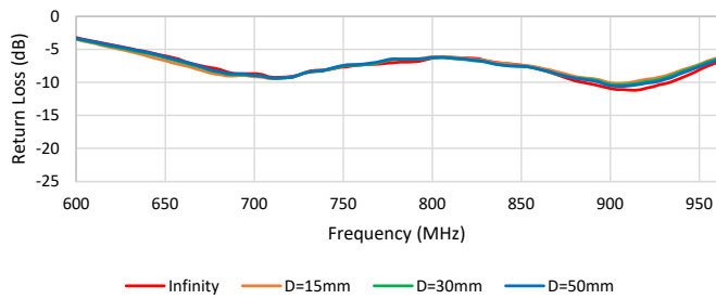
Return Loss for 2372112-1 (150mm) in Parallel Floating Metal Plate Distance (Left Side)
