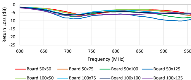
Return Loss for 2372112-2 (100mm) in Orthogonal Ground Plane Distance
