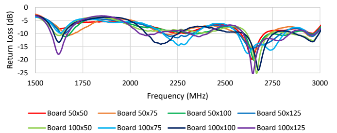
Return Loss for 2372112-2 (100mm) in Orthogonal Ground Plane Distance
