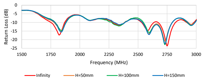
Return Loss for 2372112-1 (150mm) in Orthogonal Floating Metal Plate Distance (Centered)
