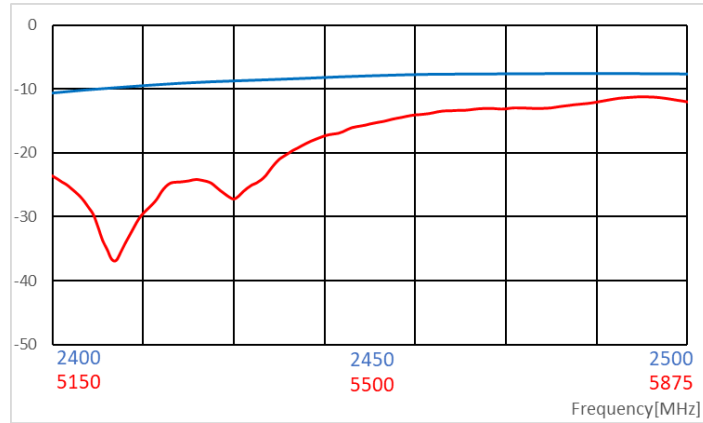
Return Loss
