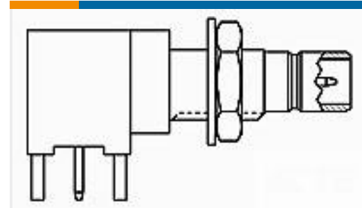
TE Part #415377-2 JACK, RATNG, PCB, SMB, 75 OHM
