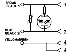
ELECTRICAL DIAGRAM A1
