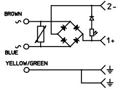
ELECTRICAL DIAGRAM S1
