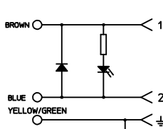
ELECTRICAL DIAGRAM C3
