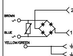
ELECTRICAL DIAGRAM S3
