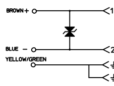
ELECTRICAL DIAGRAM S1
