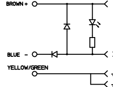
ELECTRICAL DIAGRAM 00
