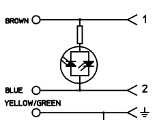
ELECTRICAL DIAGRAM A1
