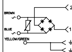
ELECTRICAL DIAGRAM S3
