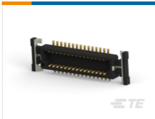
TE Part #3-5353515-0 ON TAPING (EMBOSS) 0.5MM FS CONN. TAB AS
