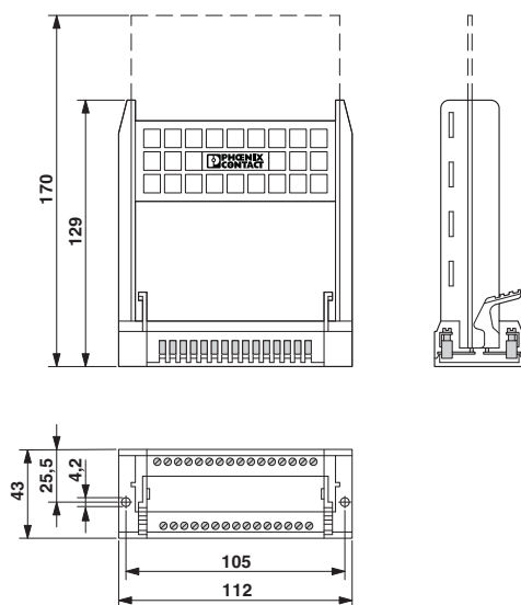
Dimensional drawing
