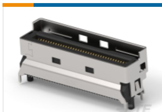
TE Part #1-2379397-7 MCIO INTERGRATED CONN, V/T, 8X, SMT TYPE
