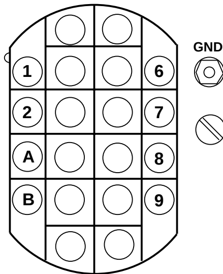
REAR VIEW OF HEADER
