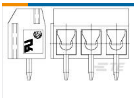
TE Part #1776266-2 2P TB ,90deg, VT, 5mm,Green,w /interlock
