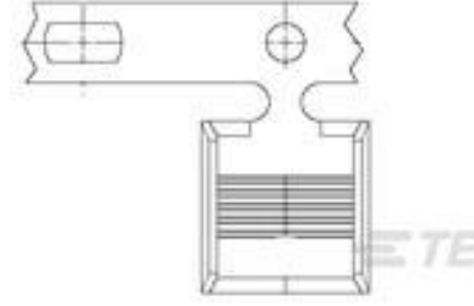
TE Part #1217990-2 AMVAR SPLC 6000-14000 025TPBR
