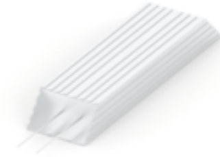
TE Part #2176509-4 CJP 400W 2R7 5% Lead
