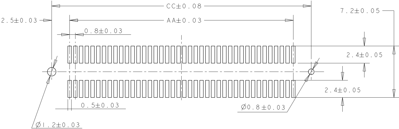
RECOMMENDED P.C.BOARD LAYOUT (REFERENCED FROM DRAWING NO. 1735480.)
