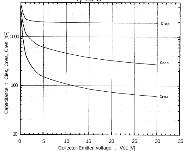
Capacitance vs. Collector-Emittor voltage
