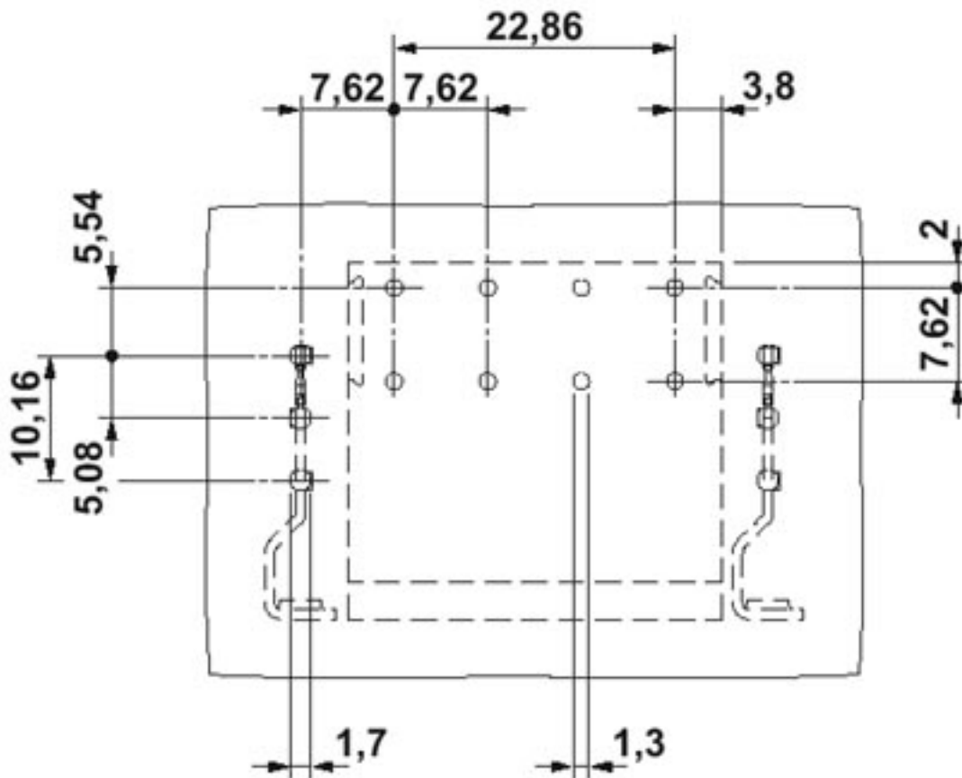
Drilling diagram
