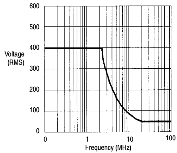
Figure 4: Typical P6139A voltage derating
