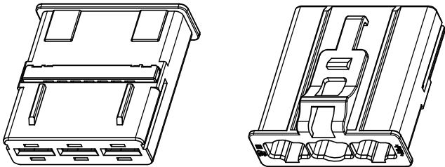
3D VIEW SCALE 1:1
