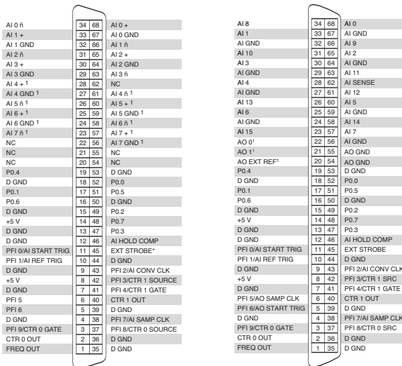
Figure 2. M Series Device Connectors
