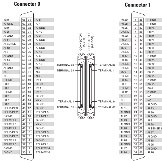
Figure 2. M Series Device Connectors
