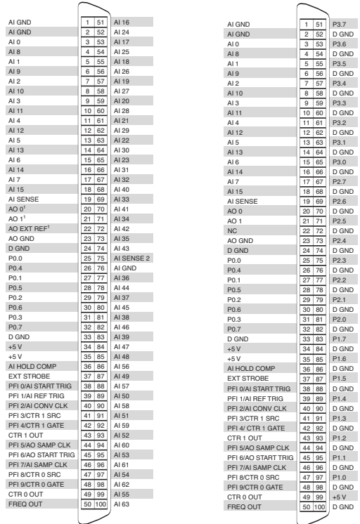
Figure 5. I/O Connector for 64-Channel E Series Devices
