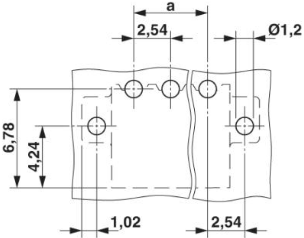
Drilling diagram
