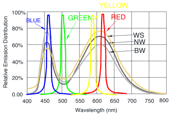
Wavelength Characteristics
