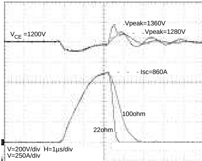
Fig.13 Effect of R_{\text{goff-SC}} in short - circuit
