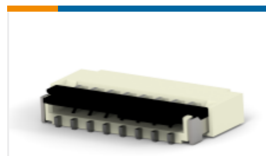
TE Part #3-2328724-1 31PIN 0.3MMP FPC CONNECTOR, FRONT FLIP
