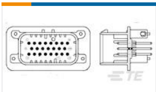
TE Part #1-776228-4 23POS, PIN DIA 1.3, HDR ASSY, 180DEG, COD 4
