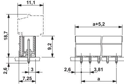
Dimensional drawing
