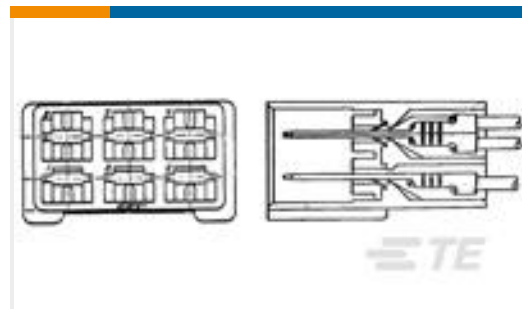
TE Part #171433-1 FF 250 TAB HSG 6P NYLON NAT
