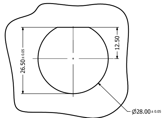
Recommended Panel Cutout ④
