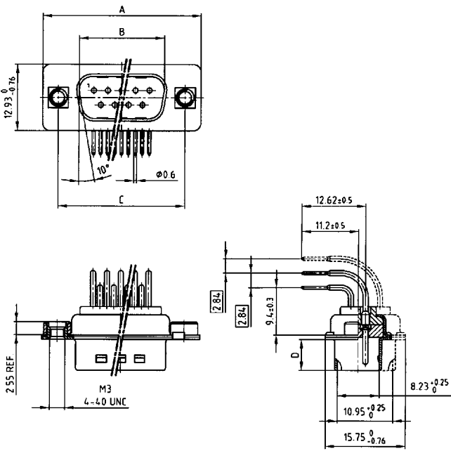
Plug connector
