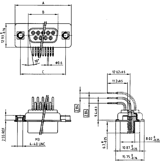
Socket connector
