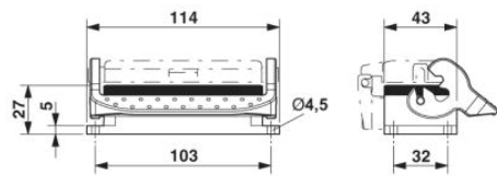
Dimensional drawing
