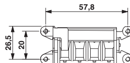
Dimensional drawing
