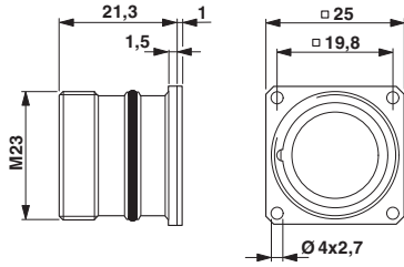
Dimensioned drawing
