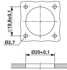
Dimensioned drawing
