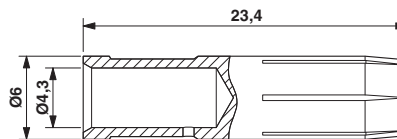
Dimensioned drawing
