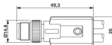
Dimensional drawing
