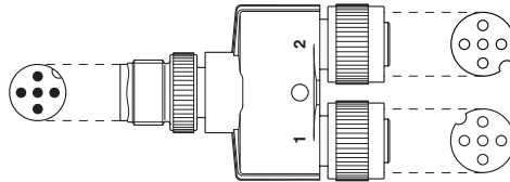
Layout of connector pin assignments
