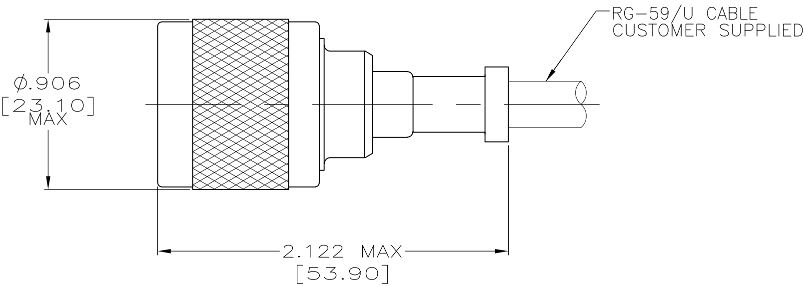
ASSEMBLED VIEW
