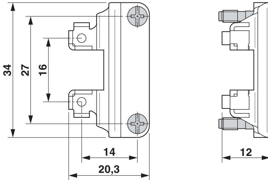
Dimensional drawing
