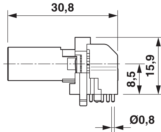
Dimensional drawing
