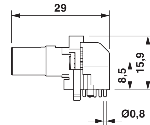
Dimensional drawing
