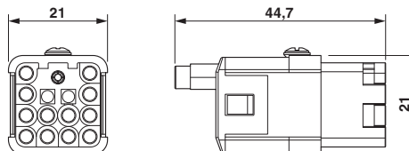
Dimensional drawing: HC-Q 12-I-CT-F
