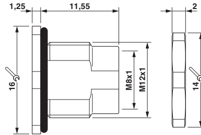
Dimensional drawing
