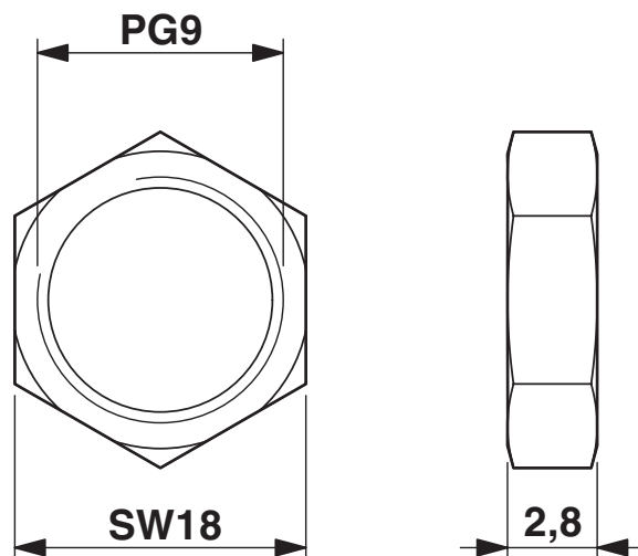
Dimensional drawing
