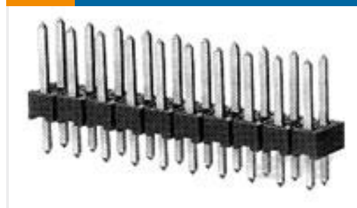
TE Part #1-826656-5 15P AMPMODU II STIFT LEI
