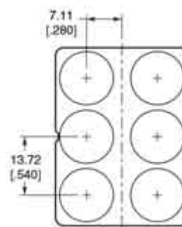
ARINC 600, 6 Position 6MS
