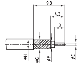
Wire stripping
