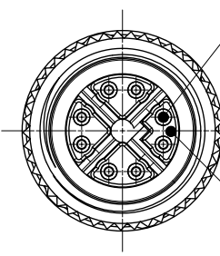
M12 X-CODE MALE FRONT VIEW
