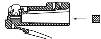
SECTION VIEW WITH NO SHIELD
